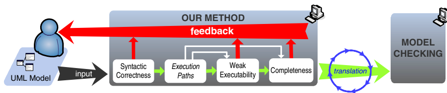
Fig. 2. Method overview
