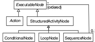
Fig. 5. Fragment of UML metamodel
